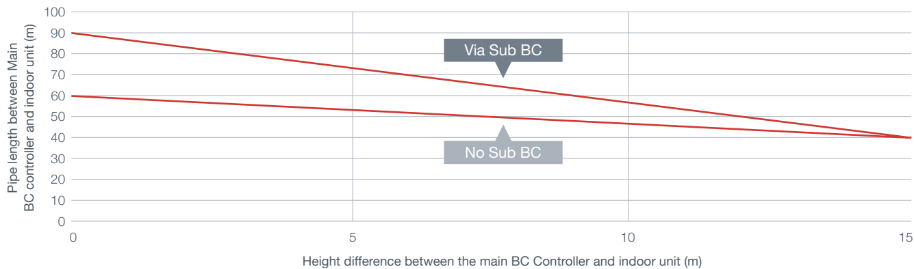
GRAPH 2: PIPE LENGTH BETWEEN BC CONTROLLER & INDOOR UNIT
